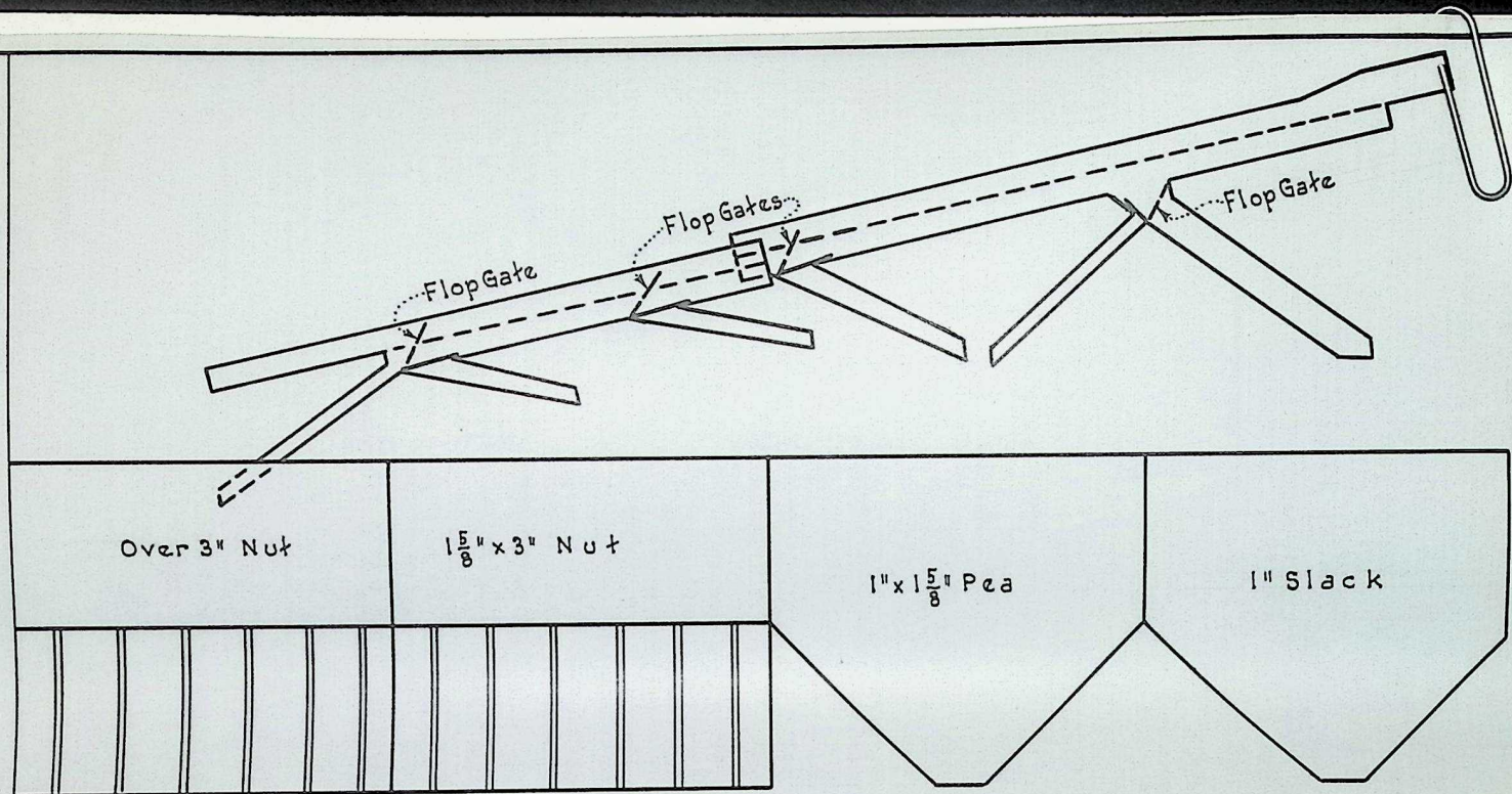
Profile Sketch CENTRAL COAL & COKE RESCREENER Central Coal & Coke Co. Rock Springs, Wyo. Not to Scale Mar. 20, 1934.
