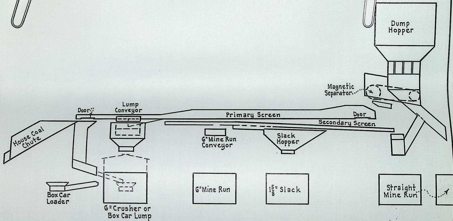
Sketch Showing PROFILE OF WINTON TIPPLE Common to No. 1 & 3 Mines Winton, Wyo. Not to Scale Aug. 15, 1934.
