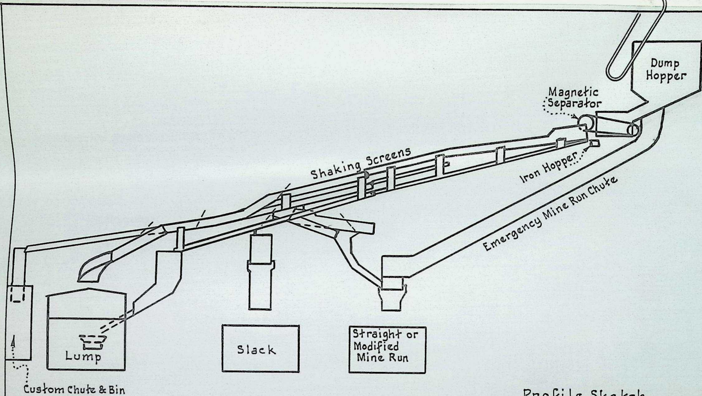
Profile Sketch No. 8 TIPPLE THE UNION PACIFIC COAL CO. Rock Springs, Wyo. Not to Scale Aug. 15, 1934.
