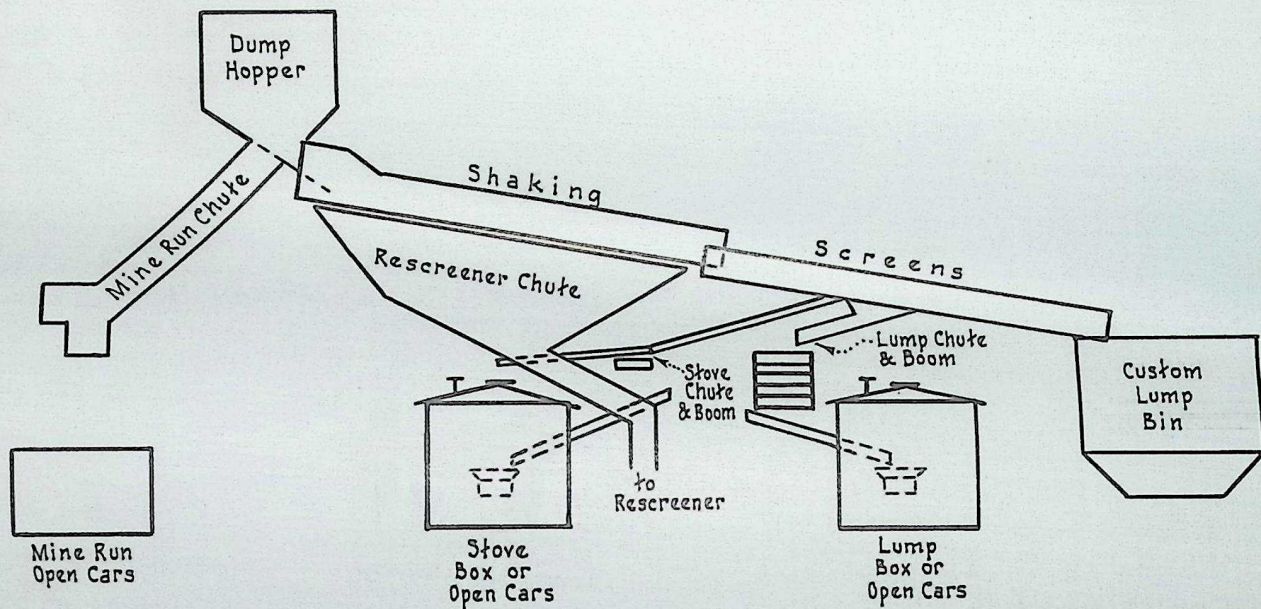
Profile Sketch MEGEATH No. 7 TIPPLE MEGEATH COAL CO. Rock Springs, Wyoming Not to Scale Aug. 25, '34.
