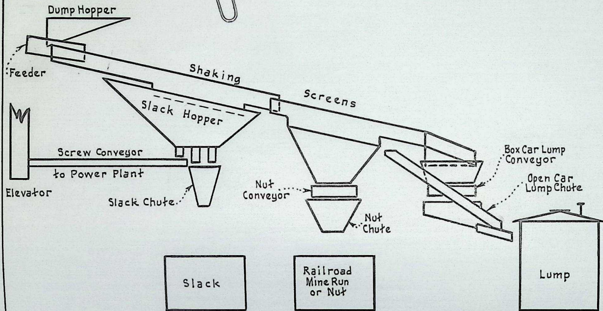
Profile Sketch OAKLEY TIPPLE DIAMOND COAL & COKE CO. Diamondville, Wyo. Not to Scale 12-14-1934.
