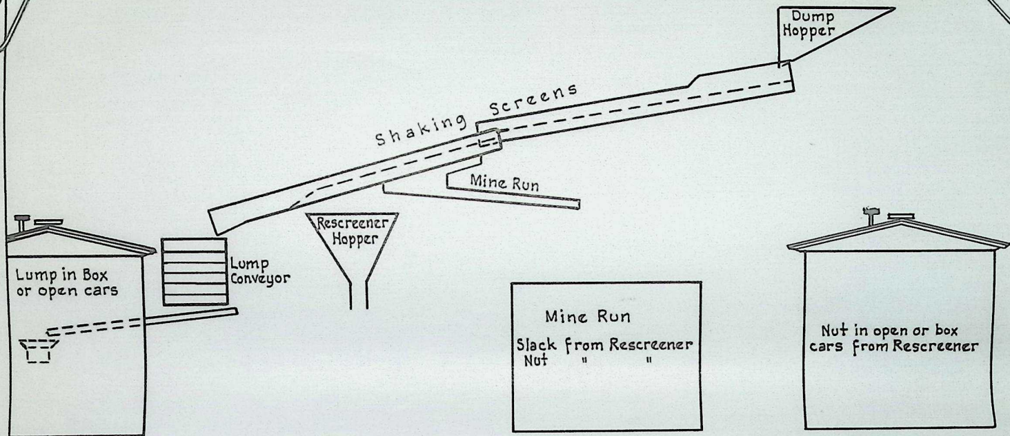
Profile Sketch CENTRAL COAL & COKE TIPPLE Central Coal & Coke Co. Rock Springs, Wyoming Not to Scale Mar. 20, 1934.
