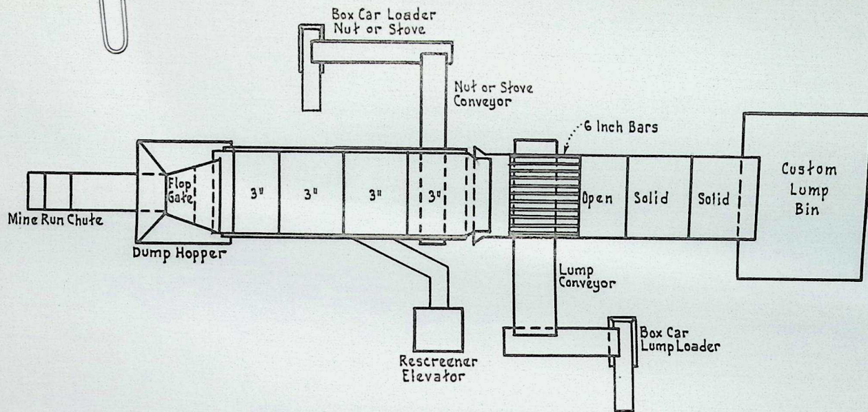
Plan Sketch MEGEATH No. 7 TIPPLE MEGEATH COAL CO. Rock Springs, Wyo. Not to Scale Aug. 25, 1934.
