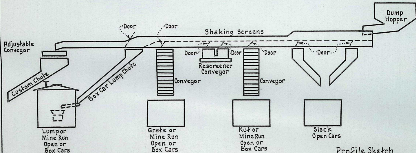
Profile Sketch DINES TIPPLE COLONY COAL Co. Dines, Wyo. Not to Scale 11-16-1934.
